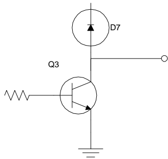
Megasquirt Fuel Pump Drive
